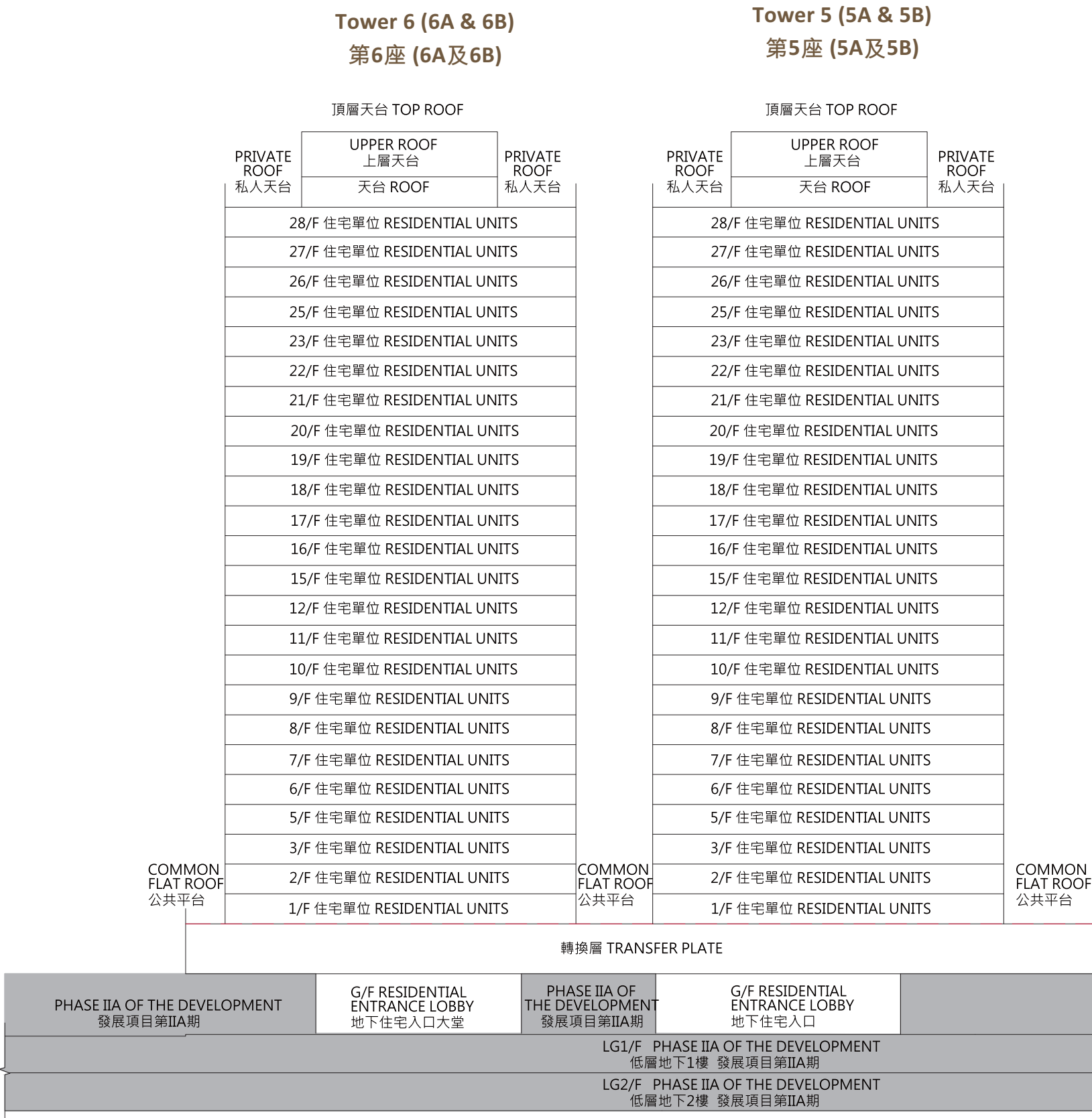
Cross-section Plan C-C 橫截面圖C-C
