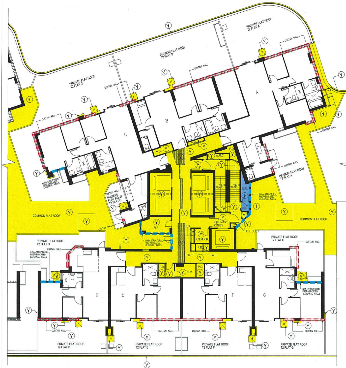
1/F PLAN OF TOWER 2
