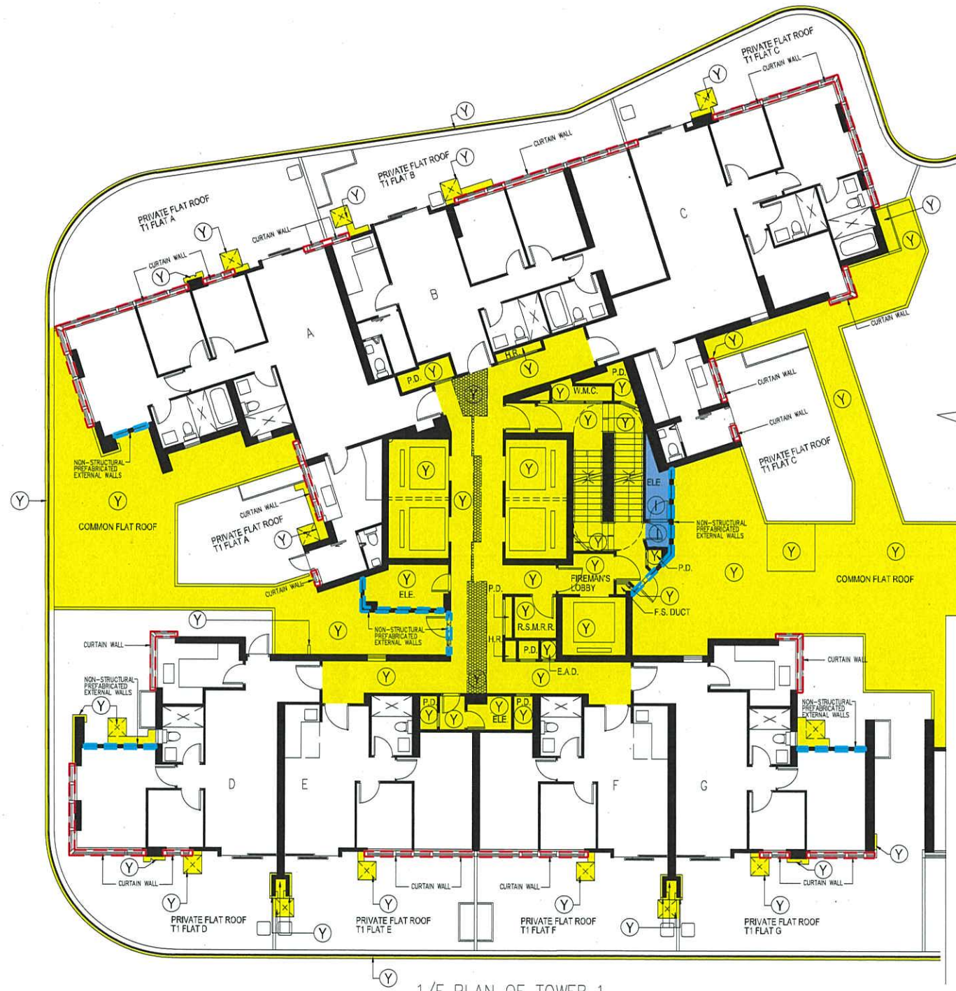
1/F PLAN OF TOWER 1
