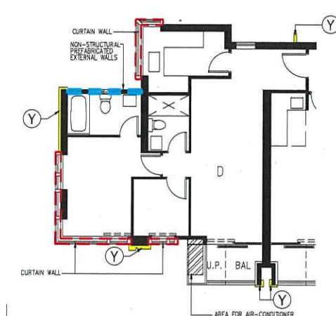
15/F FLAT D PART PLAN OF TOWER 1
