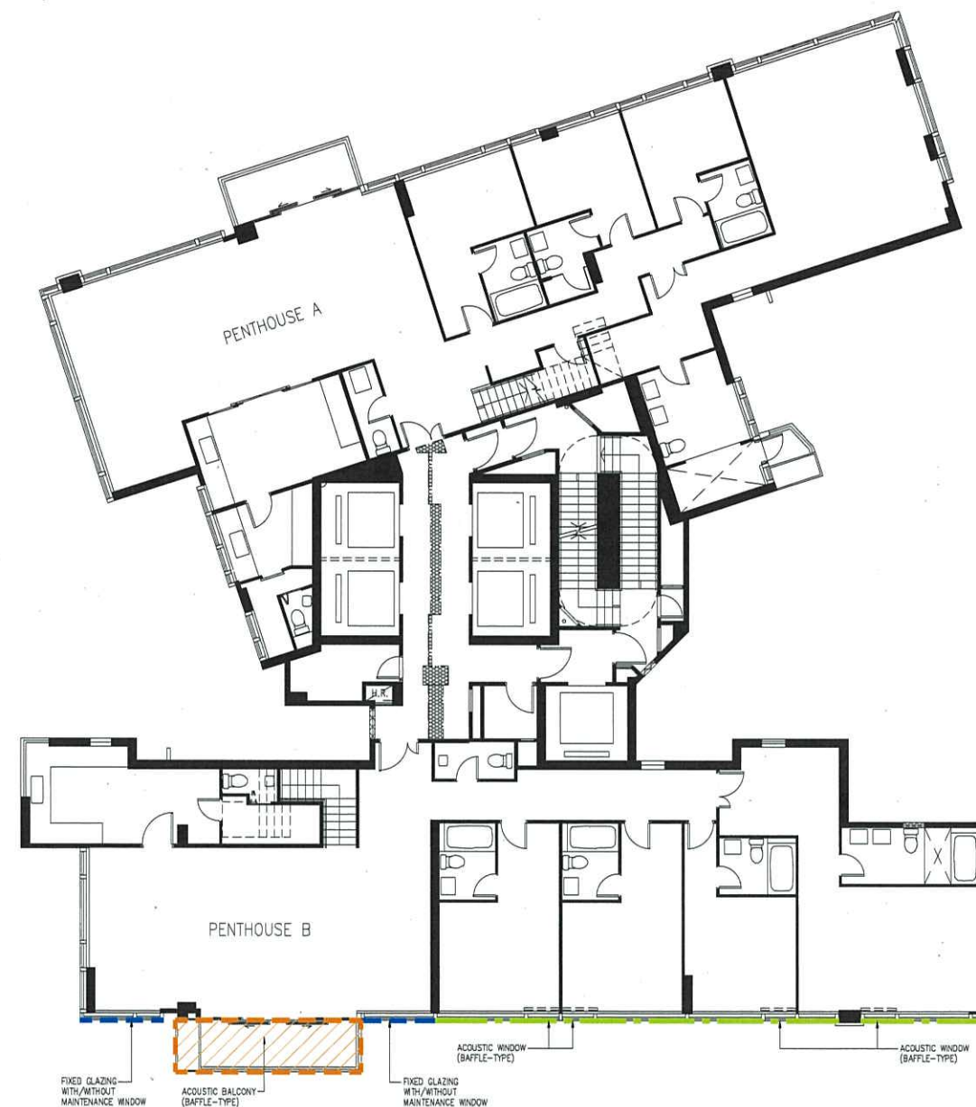
28/F PLAN OF TOWER 1
