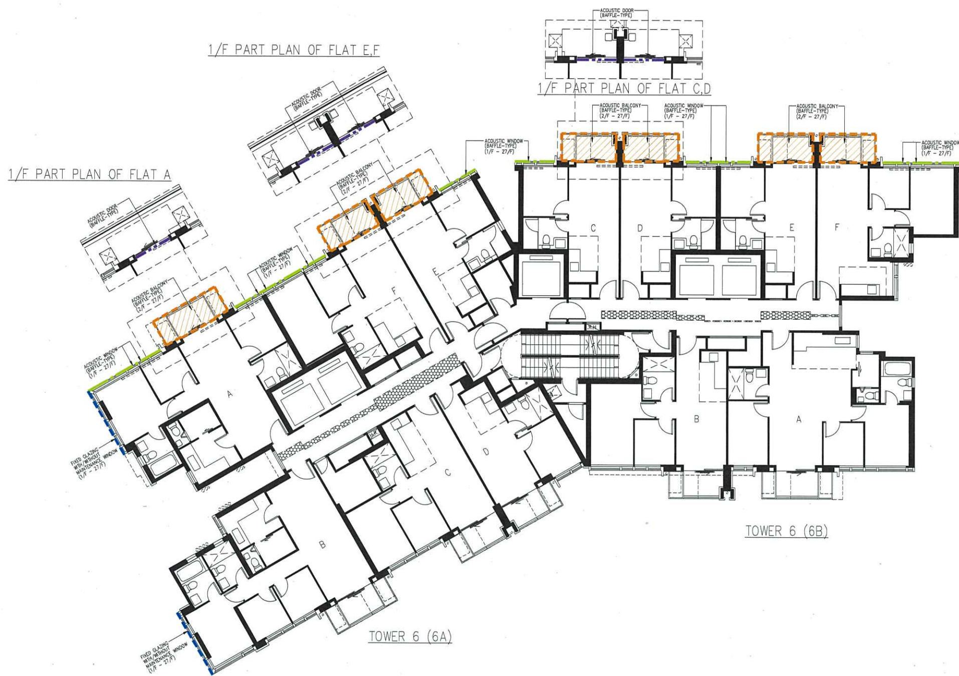
1/F-27/F PLAN OF TOWER 6 (6A&6B) (23 STOREYS) (OMITTED 4/F, 13/F, 14/F AND 24/F)
