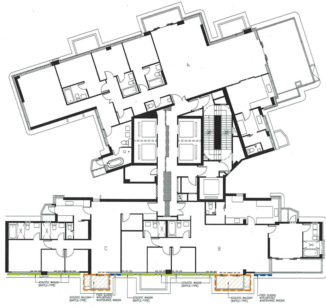
27/F PLAN OF TOWER 3
