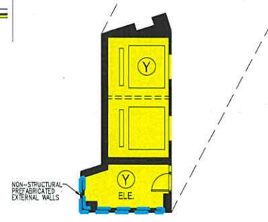
2/F PART PLAN OF TOWER 1
