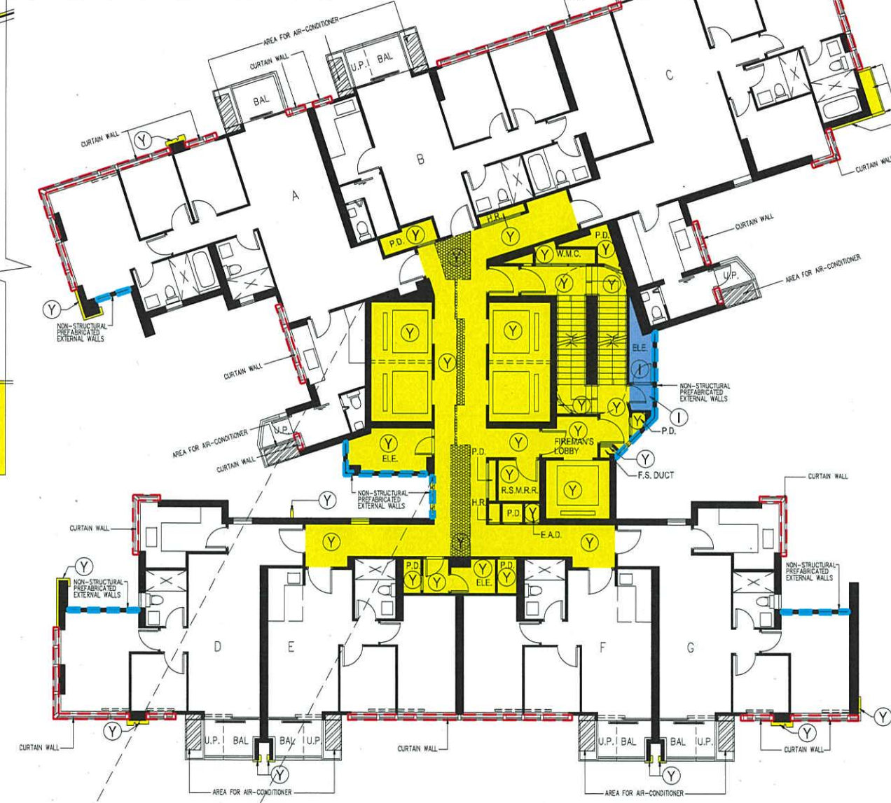
15/F FLAT D PART PLAN OF TOWER 1
