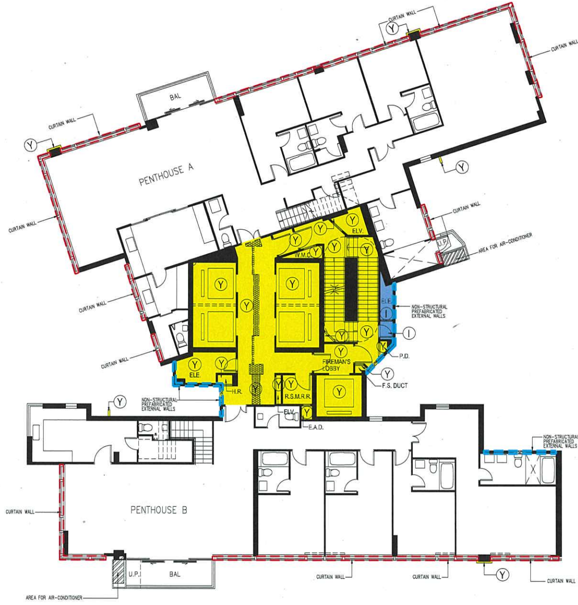
28/F PLAN OF TOWER 1
