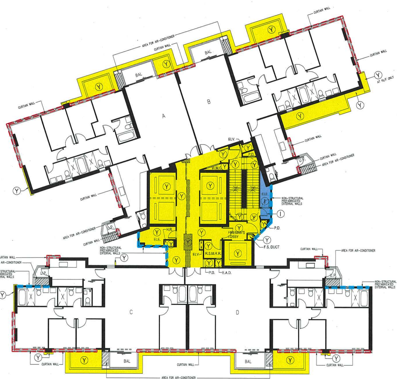
16/F-26/F PLAN OF TOWER 1 (10 STOREYS) (OMITTED 24/F)
